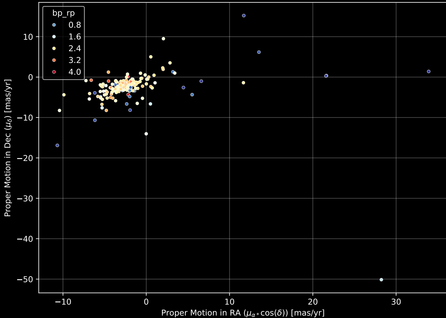
APOGEE DR17 Field: [101+04] Proper Motion Diagram (n= 194)
