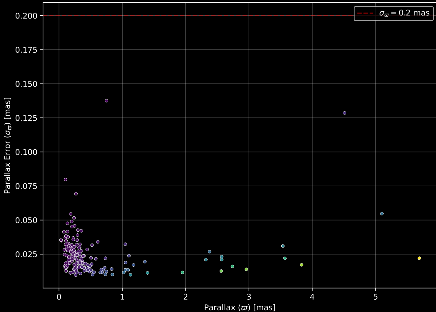
APOGEE DR17 Field: [101+04] Parallax Quality (n= 194)
