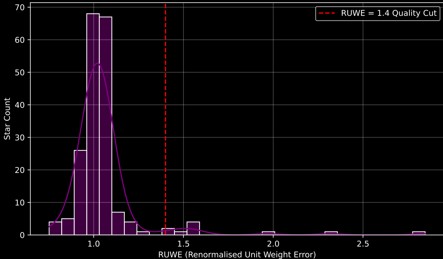
GAPOGEE DR17 Field [101+04] RUWE Distribution (n= 192)
