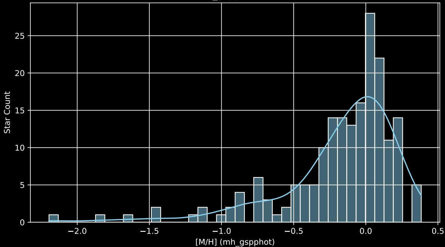
APOGEE DR17 Field: [101+04 [M/H] (mh_gspphot) (n= 189)
