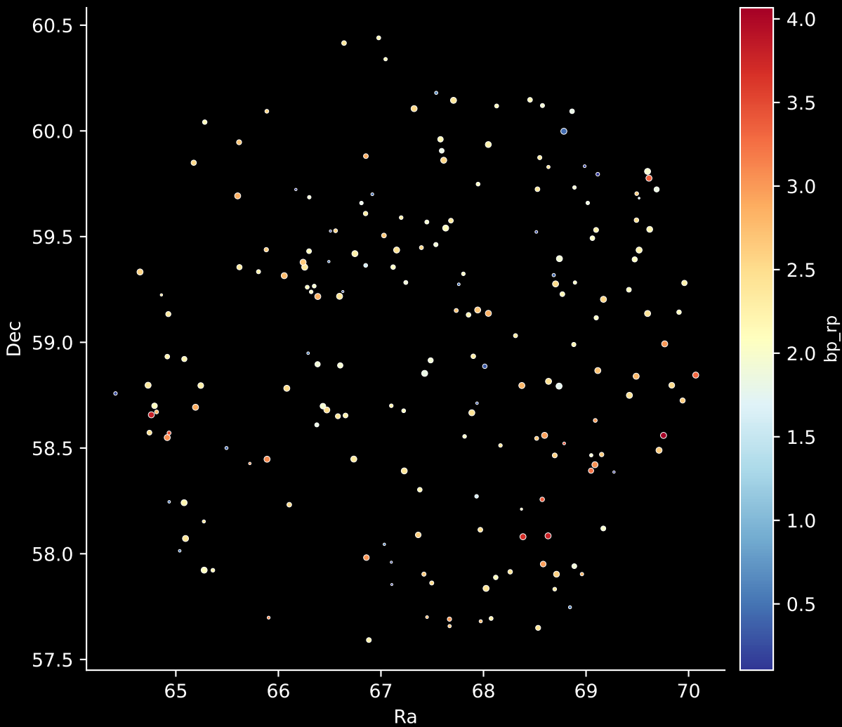
APOGEE DR17 Field: [101+04] Stars: 194
